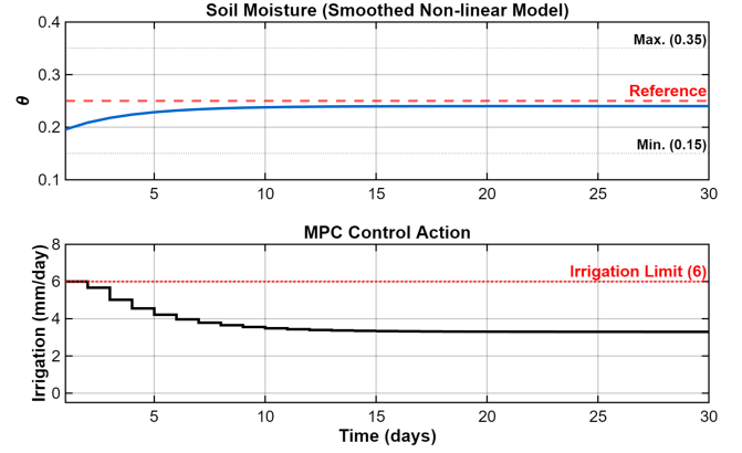
Figure 6. MPC response under smooth formulations for drainage and water stress ( K_s ).
