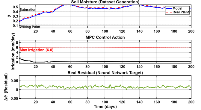
Figure 10. Synthetic data generation: (top) moisture evolution (model vs plant); (center) irrigation calculated by the MPC; (bottom) residual term target for neural network training.
